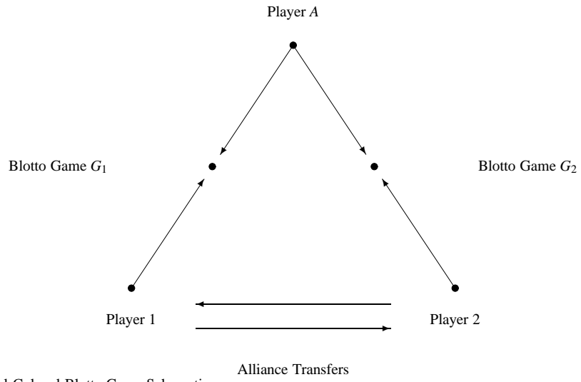
Fig. 1 Coalitional Colonel Blotto Game Schematic
